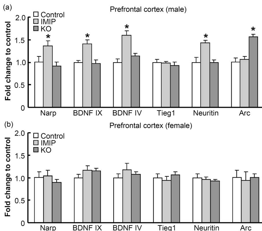
Figure 6 Seven weeks of KO administration leads to gender-specific effects on activity-regulated cytoskeleton-associated ( Arc ) mRNA regulation in the prefrontal cortex. Changes in mRNA expression following KO administration is expressed as fold change relative to the control group. (a) Male rats n=12 control, n=11-12 IMIP, n=12 KO, (b) Female rats n=11-12 control, n=8-9 IMIP, n = 14 KO. * p<0.05 from Student's t-test.
